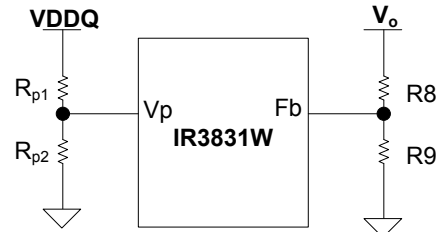
Fig. 10. Typical application of the IR3831W for programming the output voltage
