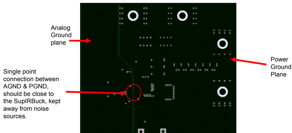
Fig. 26c. IR3831W layout considerations – Mid Layer 1
